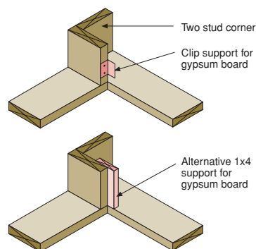
Figure 32 Corner framing
