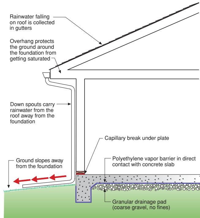
Figure 10 Capillary break over footing
